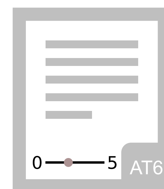
Numerical annotation
