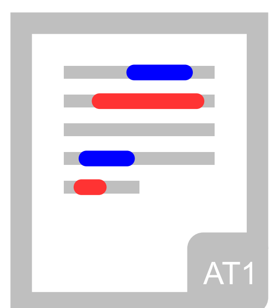
Span labeling
